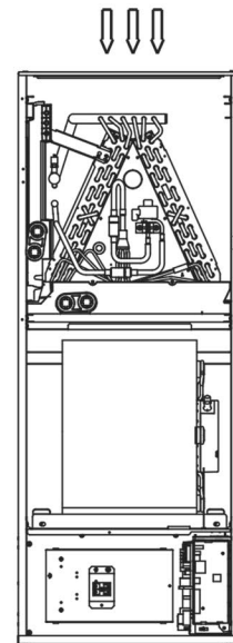
downflow
